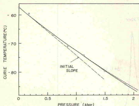
Fig. 3. Hydrostatic pressure dependence of the Curie temperature of GSN. The dott-and-slashed curve represents the initial slope. The slashed curve indicates the calculated curve from eq. (5).
